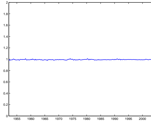
(a) \beta \exp(c_t) / \exp(c_{t+1})
