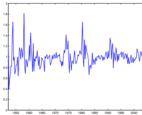
(b) g(s_{t+1} - s_t | \mathcal{S}_t)
