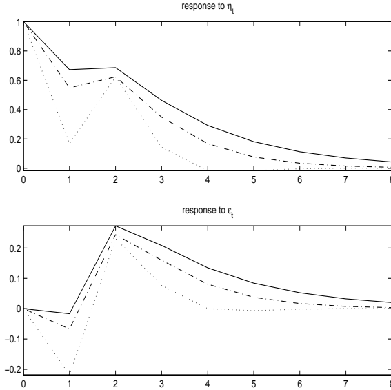
FIGURE 10. Top panel: impulse responses of inflation to the shock \eta_t under three values of \theta : \theta = +\infty (solid line), \theta = 10 (dashed-dotted line), and \theta = 5 (dotted line), with \beta = 1 . Bottom panel: impulse response of inflation to shock \epsilon_t under same three values of \theta .
