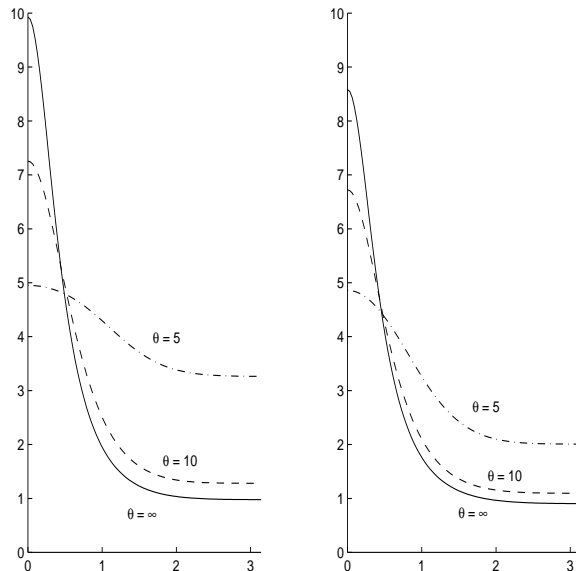
FIGURE 9. Frequency decompositions of trace [h(\omega)'h(-\omega)] for objective function of Ball's model under three decision rules; \beta = 1 on left panel, discount factor \beta = .9 on right panel.
