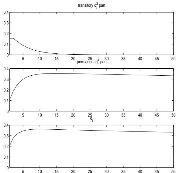
FIGURE 4. Impulse responses for two components of endowment process and their sum in Hansen, Sargent, and Tallarini's model. The top panel is the impulse response of the transitory component d^2 to an innovation in d^2 ; the middle panel, the impulse response of the permanent component d^1 to its innovation; the bottom panel is the impulse response of the sum d_t = d_t^1 + d_t^2 to its own innovation.
