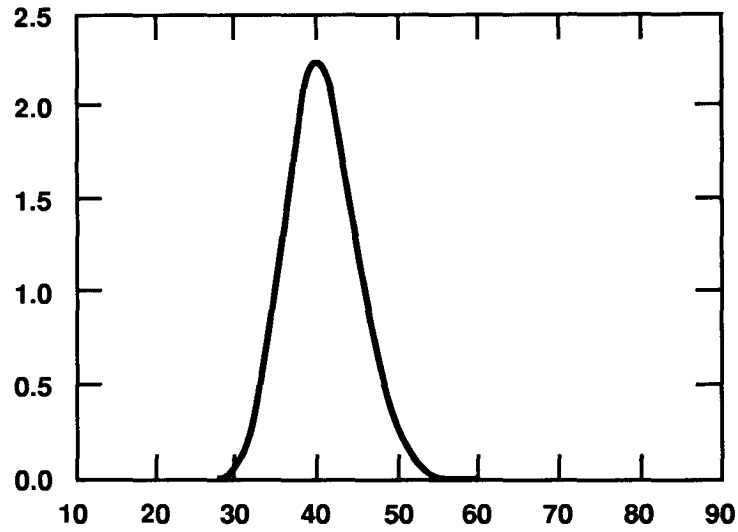
Figure 12. Density function in arbitrary units for Case VII-B.
